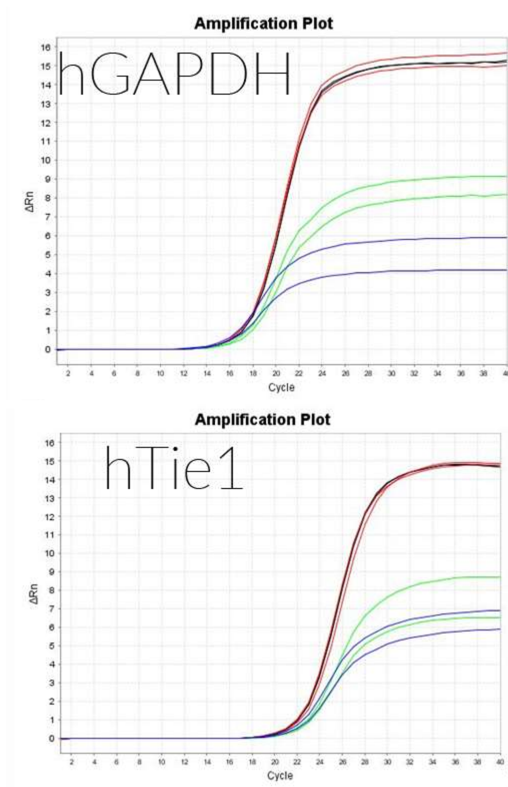
Fig.1: Comparison of FastGene ® IC Green (black & red) with the market leading competitors KB (green) and T (blue). The differences of the CT-values were under 1 cycle.
