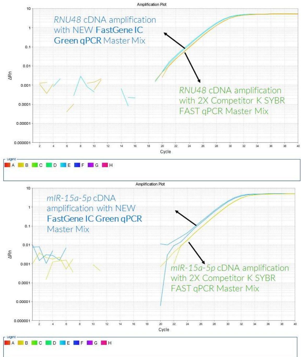
Fig. 2: Comparison of FastGene ® IC Green (blue) with the market leading competitors KB (yellow). The differences of the CT-values were under 1 cycle. Data was kindly provided by an independent researcher.
